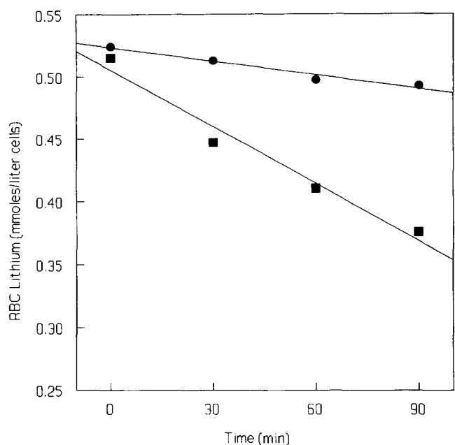
Figure 1. Plot of RBC lithium concentration versus time for a representative subject (ID 27207) during the 90-minute incubation procedure used to determine k_{exch} . Circles, data from cells incubated in sodium-free media. Squares, data from cells incubated in sodium-containing media. Lines were fitted to the two types of data by the method of least squares.
